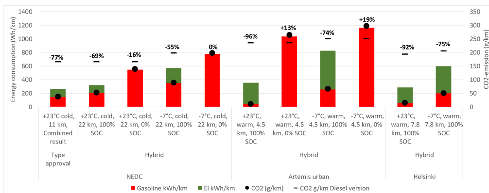
Figure 4. Vehicle A; hybrid auto drive mode CO 2 -emissions (black dots) in g/km and energy consumption (Wh/km), compared with the official type approval values. The vehicle selects by itself to drive in a Charge Depletion drive mode or a Charge Sustain drive mode. Cold = Cold start, Warm = Warm or semi-warm start depending on previous test (See schedule in Appendix A). CO 2 -emission (black hyphen) of the most comparable diesel engine version of the vehicle and emission reduction vs. diesel version (percentages) are also shown.
