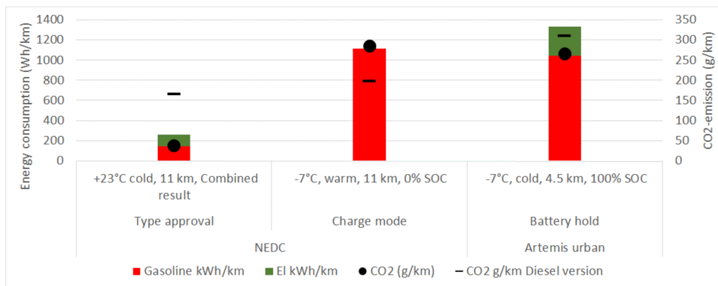
Figure 6. Vehicle A: battery hold and battery charge modes’ energy consumption (Wh/km, gasoline and electricity) and CO 2 -emission (black dots) in (g/km) compared with the NEDC official type approval values and the CO 2 emission (black hyphen) of the diesel version of the same vehicle. The batter charge mode is used to increase the SOC of the battery while driving. Battery hold mode keeps the battery SOC at the present value. Cold = Cold start, Warm = Warm or semi-warm start depending on previous test (See schedule in Appendix A).
